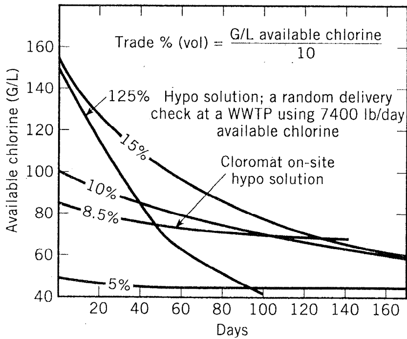
Fig. 2-1. Decay rate sodium hypochlorite solutions.
